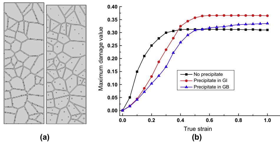
Fig. 6. Computational model of UFG titanium with precipitates in grain boundary phase and in grain interior (a) and the effect of the precipitate distribution on the damage evolution in UFG titanium (b). (Reprinted from [76,77] with kind permission from Elsevier).
