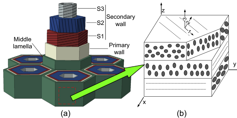
Fig. 2. Multiscale model of wood as layered, cellular (a) and fibril reinforced (b) material [24,25] (Reprinted with kind permission from Elsevier). The thin layers S1, S3 with fibrils perpendicular to the fibrils in thick S2 layer control the buckling and fracture resistance.
