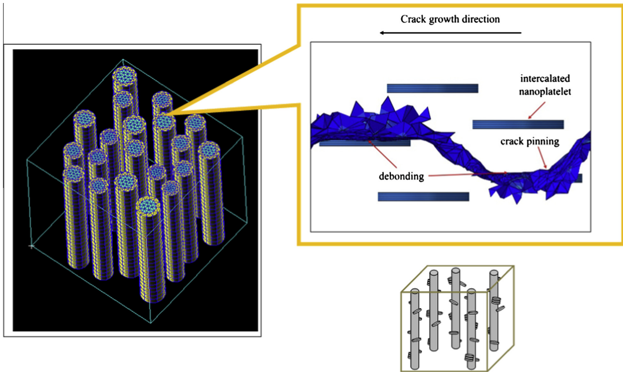
Fig. 5. Crack propagation in the fiber sizing of hierarchical composite (result of FE simulations). Right below – schema of hierarchical fiber reinforced composite with secondary nanoplatelet (Reprinted from [39,61] with kind permission from Elsevier).
