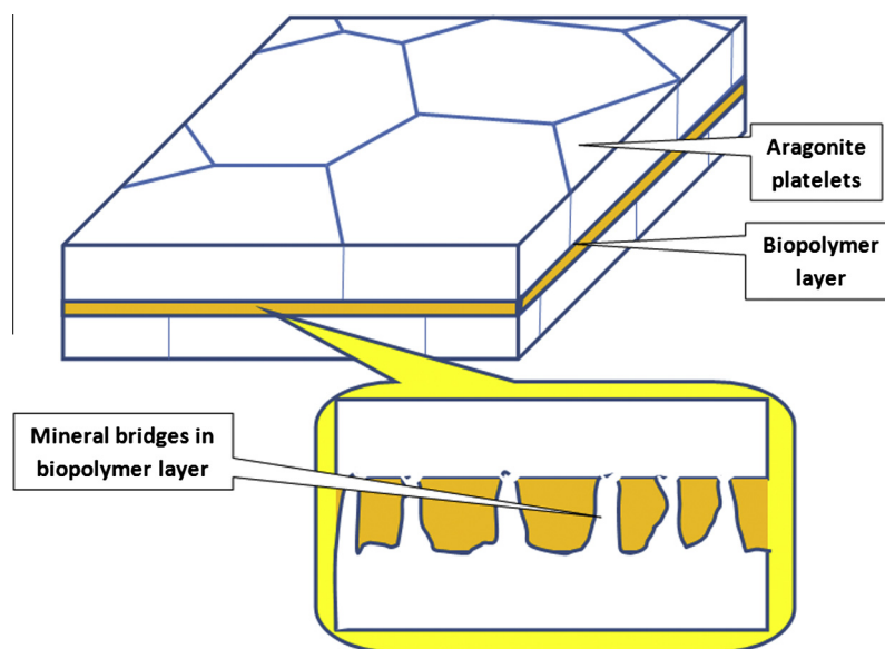
Fig. 1. Schema of microarchitecture of nacre: aragonite platelets, biopolymer layer and mineral bridges (after [16,17]).
