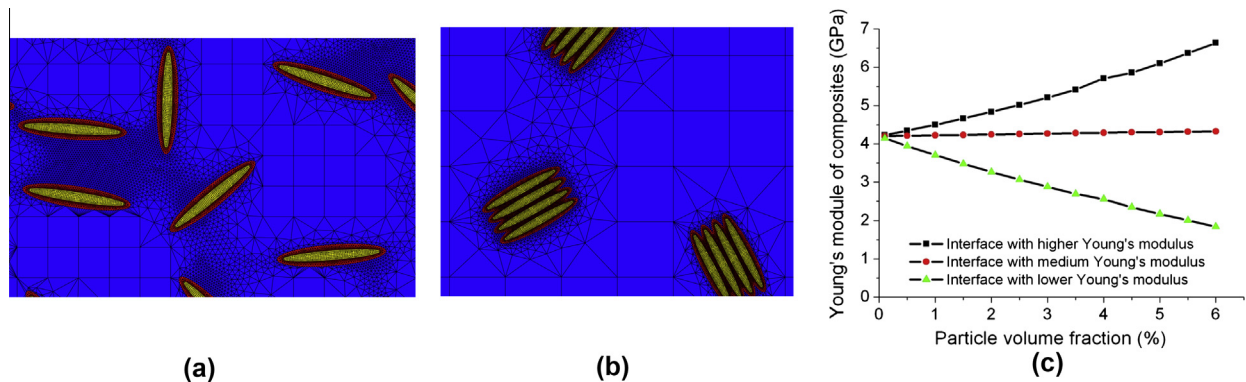
Fig. 4. Generalized equivalent interface (GIF) model for the analysis of nanoparticles in polymers (a and b) Finite element models with GEIF for exfoliated and intercalated (clustered) structures of nanocomposites, and (c) Effect of GIF properties on the properties of nanocomposite. (Reprinted from [43,44] with kind permission from Elsevier).
