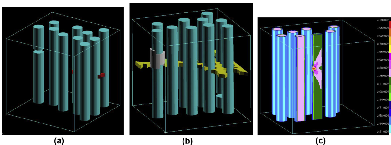
Fig. 3. Simulated damage mechanism in fiber reinforced polymer composites: Competition of damage mechanisms. (Reprinted from [29] with kind permission from Elsevier). (a and b) Interface is damaged (red region) in a region far from the first cracked fiber; matrix crack is formed far from the region with damaged interface. (c) Stress in a fiber is lower than in other fibers if its sizing is pre-damaged (For interpretation of the references to colour in this figure legend, the reader is referred to the web version of this article.).
